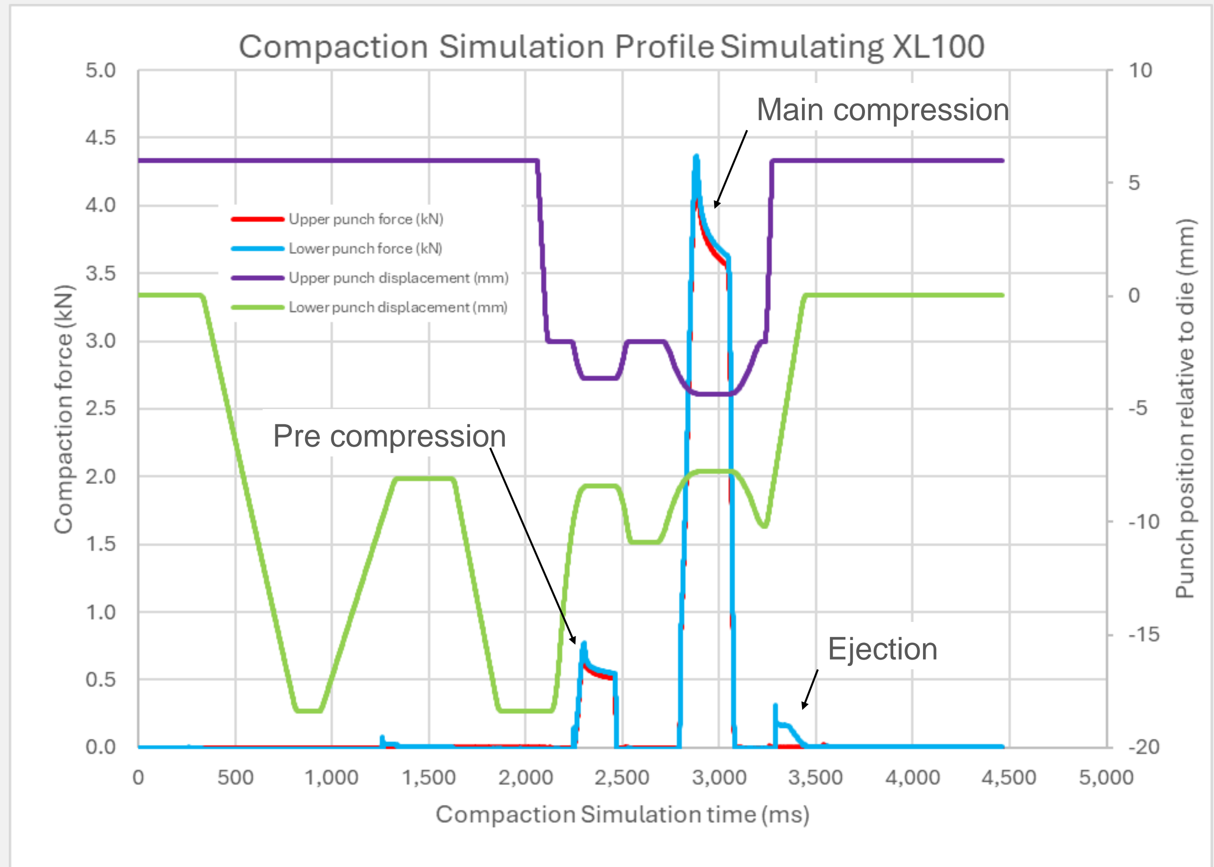
Figure 2: The compaction profile of a KORSCH XL 100 R & D rotary press simulated on the STYL'One Evo Compaction Simulator. The precompression, main compression, and ejection forces are illustrated in the lower punch force trace.
