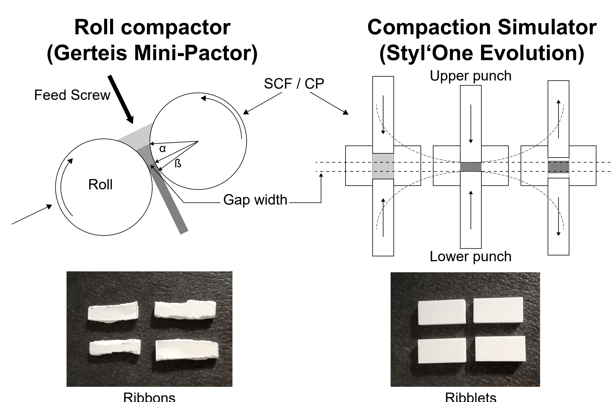
Figure 1: Principle of hybrid modeling; SCF = specific compaction force, CP = compression pressure [1]
