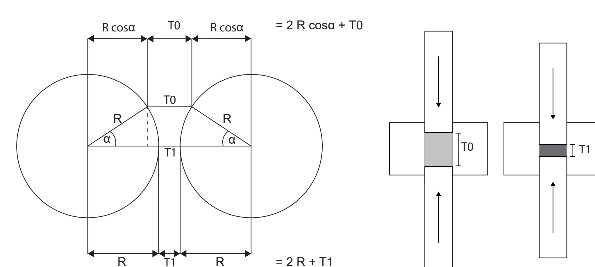
Figure 2: Principle of the nip angle determination with a uniaxial compaction simulator
