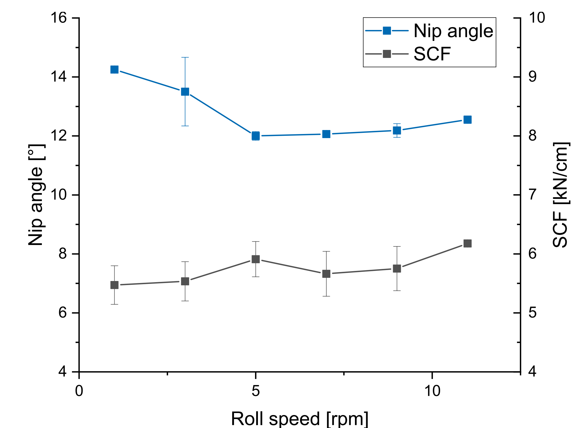
Figure 5: Nip angle of MCC depending on the roll speed at 3 mm gap width and a specific compaction force of 6 kN/cm
