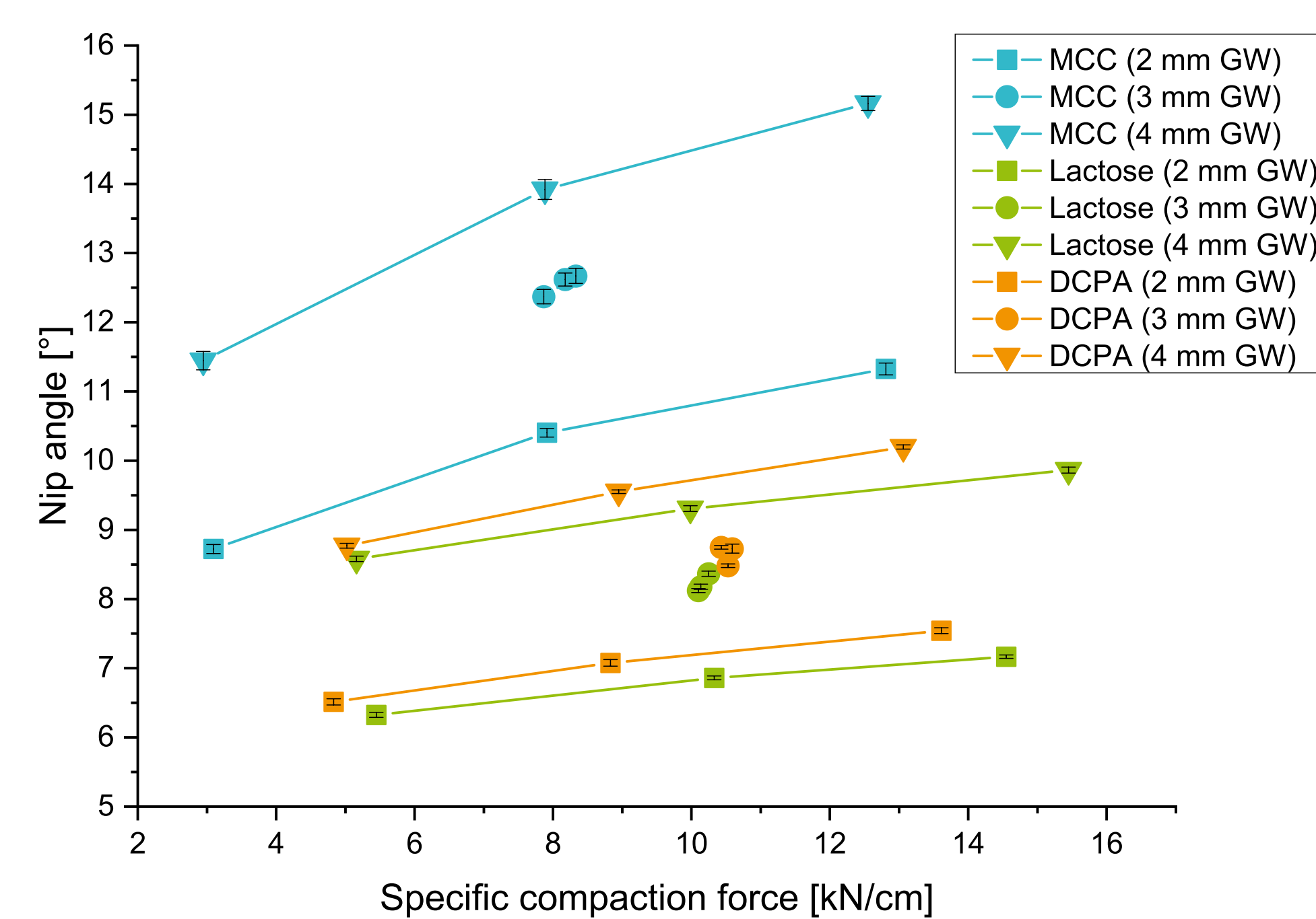
Figure 3: Nip angles of MCC, lactose and DCPA as a function of SCF at a roll speed of 2 rpm ( n \geq 20 ; mean \pm SD)
