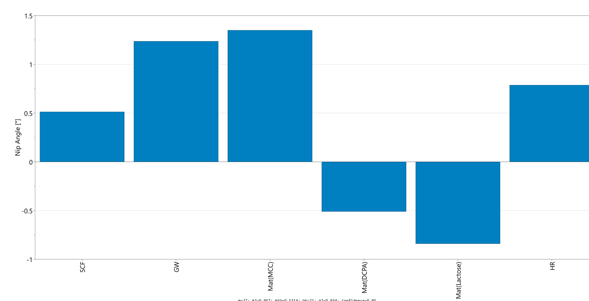
Figure 4: Coefficient plot - effects of specific compaction force (SCF), gap width (GW) Hausner ratio (HR) and material on the nip angle
